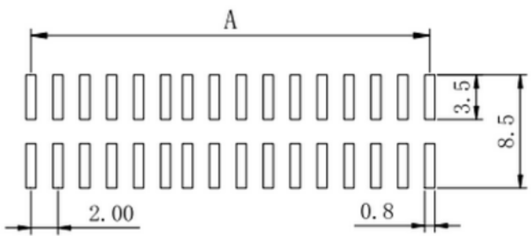
PCB LAYOUT
